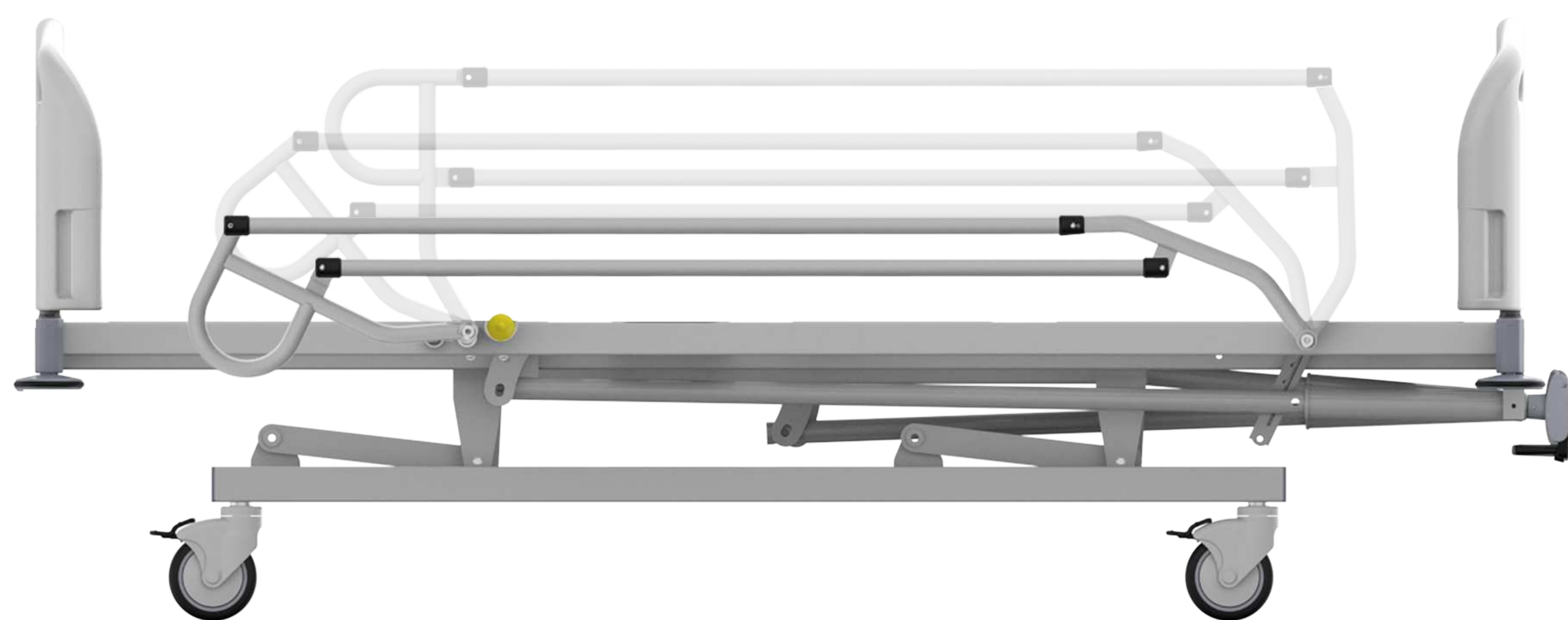
30° Legrest Movement
